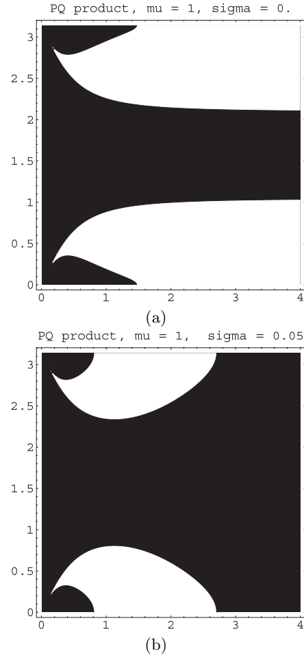
Fig. 1. The PQ = 0 curve is represented against normalized wavenumber k/k_D (horizontal axis) and angle \theta (vertical axis); the area in black (white) represents the region in the (k - \theta) plane where the product is negative (positive), i.e. where the wave is stable (unstable). This plot refers to the dust-free case ( \delta = 0 i.e. \mu = 1 ). (a) \sigma = 0 (cold ions); (b) \sigma = 0.05 (warm ions).
