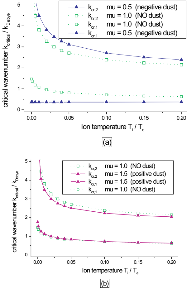
Fig. 4. The two critical wavenumber values k_{cr,1}/k_{cr,2} are depicted (lower/upper solid line, triangles) against normalized ion temperature \sigma = T_i/T_e , for a dusty plasma with negative dust charge. The unstable region lies between the two curves. The dust-free case k_{cr,1}/k_{cr,2} thresholds (lower/upper dot line, squares) is also depicted, for reference. (a) Negative dust: \delta = q_{d,0}/q_{i,0} = 0.5 i.e. \mu = 0.5 ; (b) positive dust: \delta = 0.5 i.e. \mu = 1.5 . See that the addition of negative (positive) dust results in a wider (narrower) instability region, which gets even narrower with temperature, in both case.
