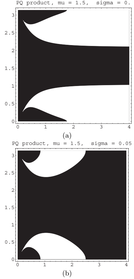
Fig. 3. Similar to the previous figures, for positive dust charge; we have taken a positive dust density: \delta = q_{d,0}/q_{i,0} = 0.5 i.e. \mu = 1.5 here.
