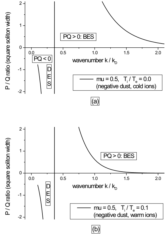
Fig. 6. Similar to the previous figure, for negative dust charge; we have taken a negative dust density: \delta = q_{d,0}/q_{i,0} = 0.5 i.e. \mu = 0.5 here.
