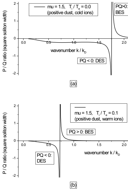
Fig. 7. Similar to the previous two figures, for positive dust charge; we have taken a positive dust density: \delta = q_{d,0}/q_{i,0} = 0.5 i.e. \mu = 1.5 here.
