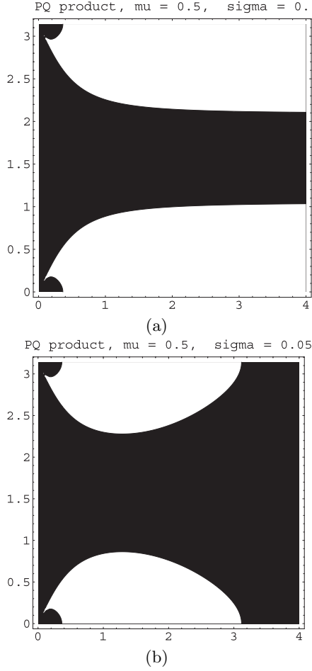
Fig. 2. Similar to the previous figure, for negative dust charge; we have taken a negative dust density: \delta = q_{d,0}/q_{i,0} = 0.5 i.e. \mu = 0.5 here.
